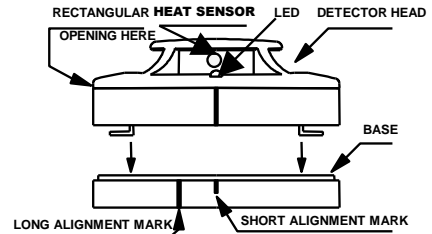
Fig. 2 Fitting detector head onto base
