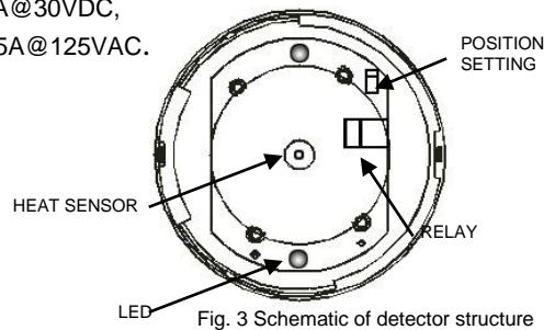
Fig. 3 Schematic of detector structure When front cover is open.
